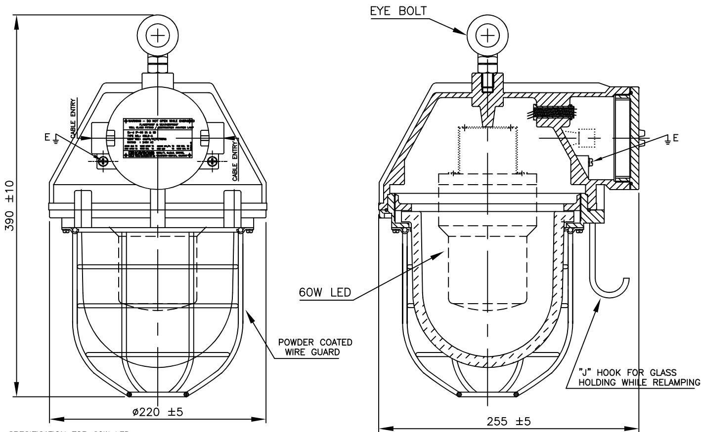
SPECIFICATION FOR 60W LED
